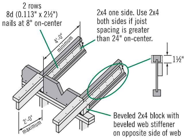
R8 Birdsmouth cut allowed at low end of joist only
